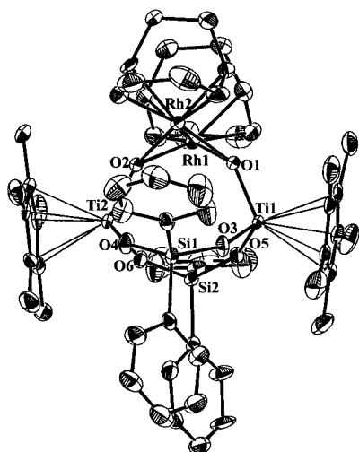
Figure 1. Structure of complex 2 . Selected bond lengths [Å] and angles ^\circ : Ti1–O1 1.796(6), Ti1–O3 1.847(6), Ti1–O5 1.860(6), Ti2–O2 1.784(6), Ti2–O4 1.846(6), Ti2–O6 1.863(6), Rh1–O1 2.135(6), Rh1–O2 2.145(6), Rh1–Rh2 2.746(1), Si1–O3 1.612(6), Si1–O4 1.625(6); O1–Rh1–O2 78.8(2), O1–Ti1–O3 104.5(3), Ti1–O1–Rh2 134.0(3), Ti1–O1–Rh1 125.1(3), Ti2–O2–Rh2 131.9(3), Ti2–O2–Rh1 130.7(3), Rh2–O1–Rh1 80.3(2).
